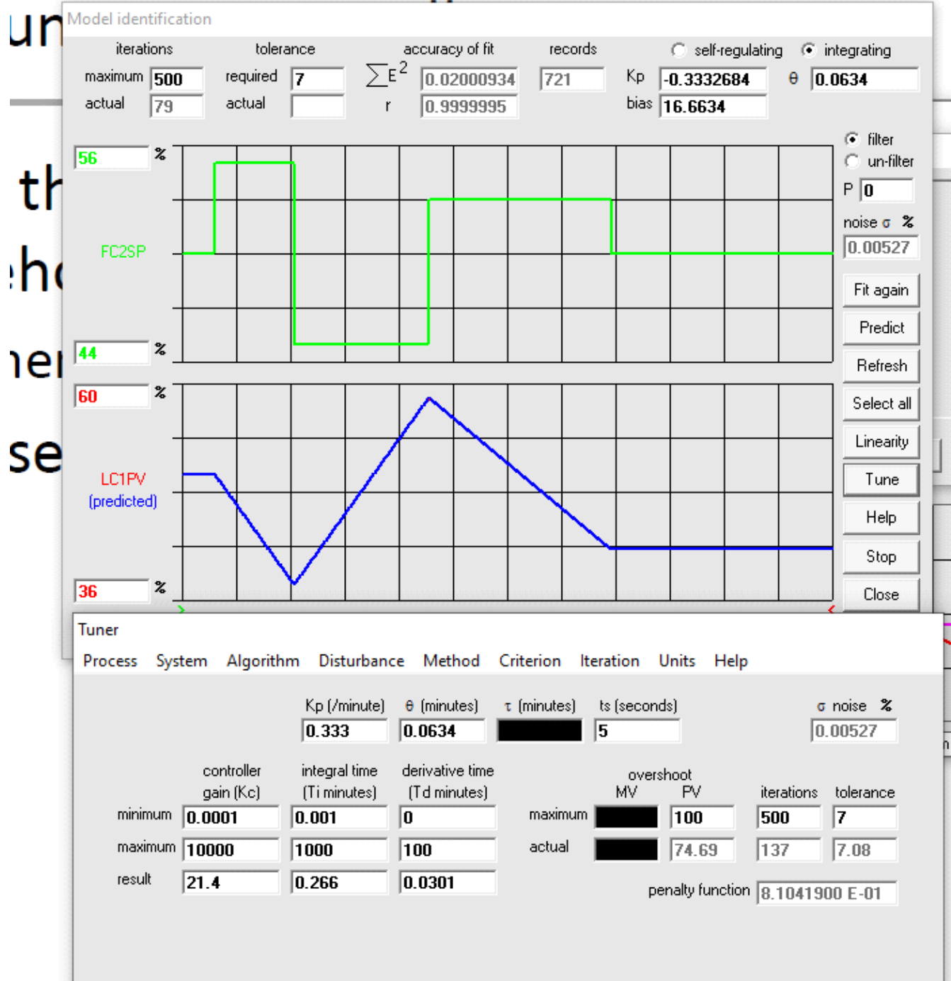
Whitehouse method by using toolkit (PID)
