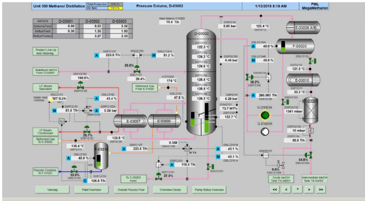
D3002 Level Commissioning
