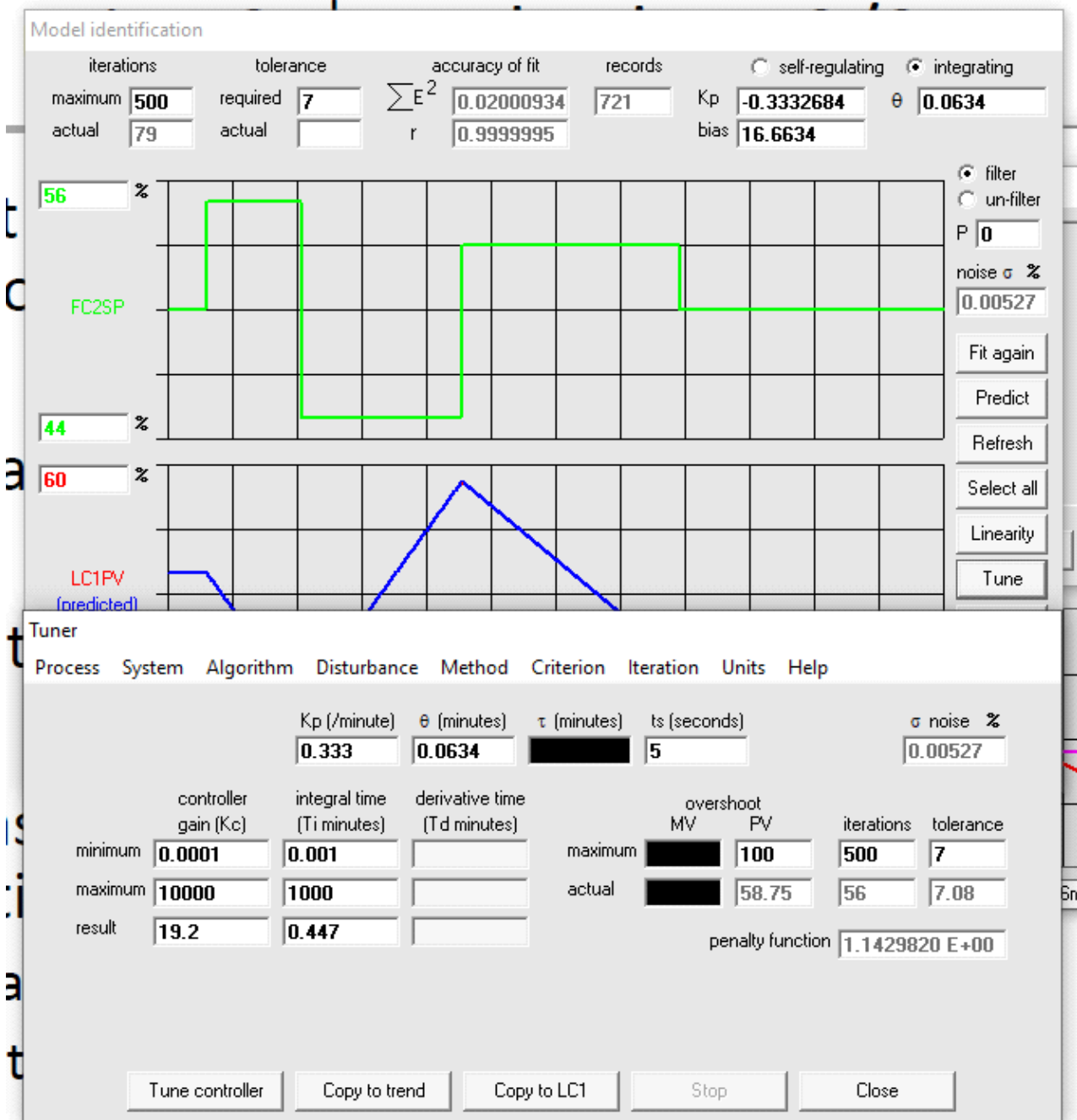
Whitehouse method (PI controller)
